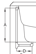
Drain/Overflow
