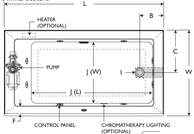
(Right End Drain / Left Side Pump) 8 WHIRLPOOL JETS
