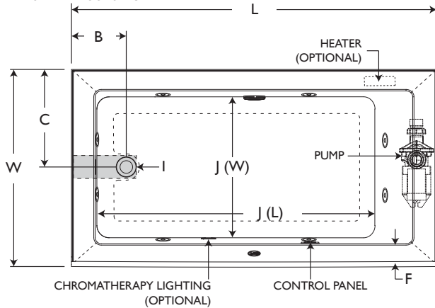
(Left End Drain / Right Side Pump) 8 WHIRLPOOL JETS
