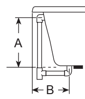
DRAIN/OVERFLOW
